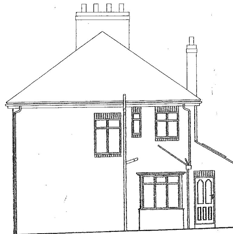
EXISTING SIDE 1:100
